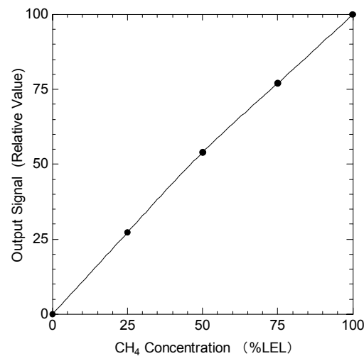
Fig 1 Sensitivity characteristic
