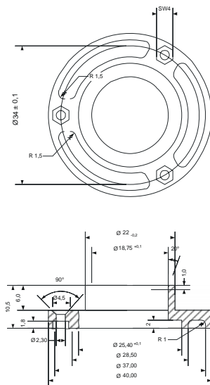
Figure 8. ECO-Sure CO sensor dimensions
