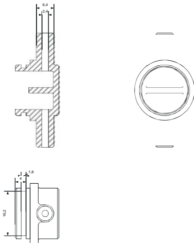
Figure 11. Test gas cap
